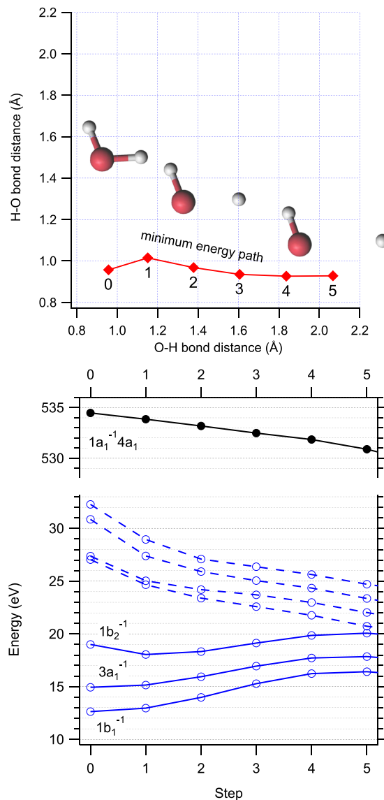
FIG. 1. (Top) The minimum energy path along the potential energy surface of 1a_1^{-1}4a_1 core-excited state. The x-axis and y-axis are the two bond distances, respectively. Step 0 corresponds to the (slightly distorted, see text) experimental ground-state geometry. The geometry for each step 1–5 corresponds to the geometry that has the minimum energy within a fixed hypersphere around the previous geometry. The result is an asymmetrical bond elongation. The bond angle (not displayed) changes by less than 2° from the ground-state geometry. (Bottom) The calculated energies of the core-excited state (black line) and several ionic final states (blue lines) corresponding to steps 0–5. The three lowest ion states (solid blue lines) are the bonding 1b_1^{-1} , 3a_1^{-1} , and 1b_2^{-1} states. The higher states (dashed blue lines) are examples chosen from an ensemble of spectator anti-bonding ion states.
