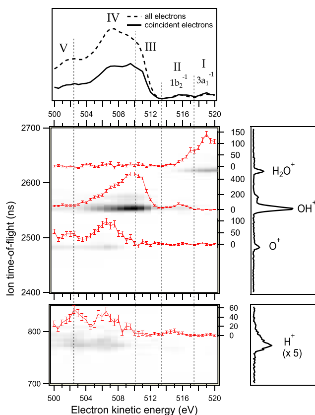
FIG. 2. Electron–ion coincidence map measured on top of the 4a_1 resonance. (Top) The resonant Auger electron spectrum showing both all electrons and those electrons detected in coincidence with ions. (Right) The coincident ion TOF spectrum. (Left) Electron–ion coincidence map. Solid red lines show coincident ion yields (CIYs) for all fragments. The ticks for the CIYs are arbitrary, but comparable, units.
