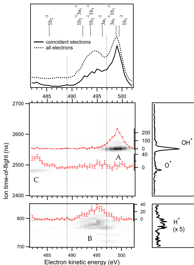
FIG. 4. Electron-ion coincidence map measured at 550 eV photon energy. (Top) The non-resonant Auger electron spectrum showing both all electrons and those electrons detected in coincidence with ions. Calculated transition energies from the 1a 1 -1 core-ionized state to the final H 2 O 2+ states are also shown. (Right) The coincident ion TOF spectrum. (Left) Electron-ion coincidence map. Solid red lines show coincident ion yields (CIYs) for all fragments. The ticks for the CIYs are arbitrary, but comparable, units.
