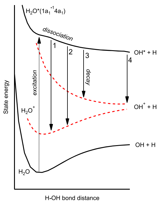
FIG. 3. A schematic illustration of the excitation, dissociation, and possible resonant Auger decay channels. The neutral ground state and the neutral core-excited state are shown in black lines, while \text{H}_2\text{O}^+ states are shown in red dashed lines. The molecule is excited from the \text{H}_2\text{O} ground state to the core-excited \text{H}_2\text{O}^*(1a_1^{-1}4a_1) state, where it starts to dissociate along the potential energy surface. The possible decay patterns are (1) prompt decay to a bonding ion \text{H}_2\text{O}^+ state, (2) later decay to a bonding ion state, (3) decay to an anti-bonding dissociative ion state, and (4) late decay where the fragmented \text{OH}^* + \text{H} ensemble decays to \text{OH}^+ + \text{H} .
